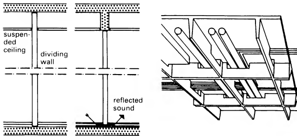
4 Floor and ceiling connections for partitions
